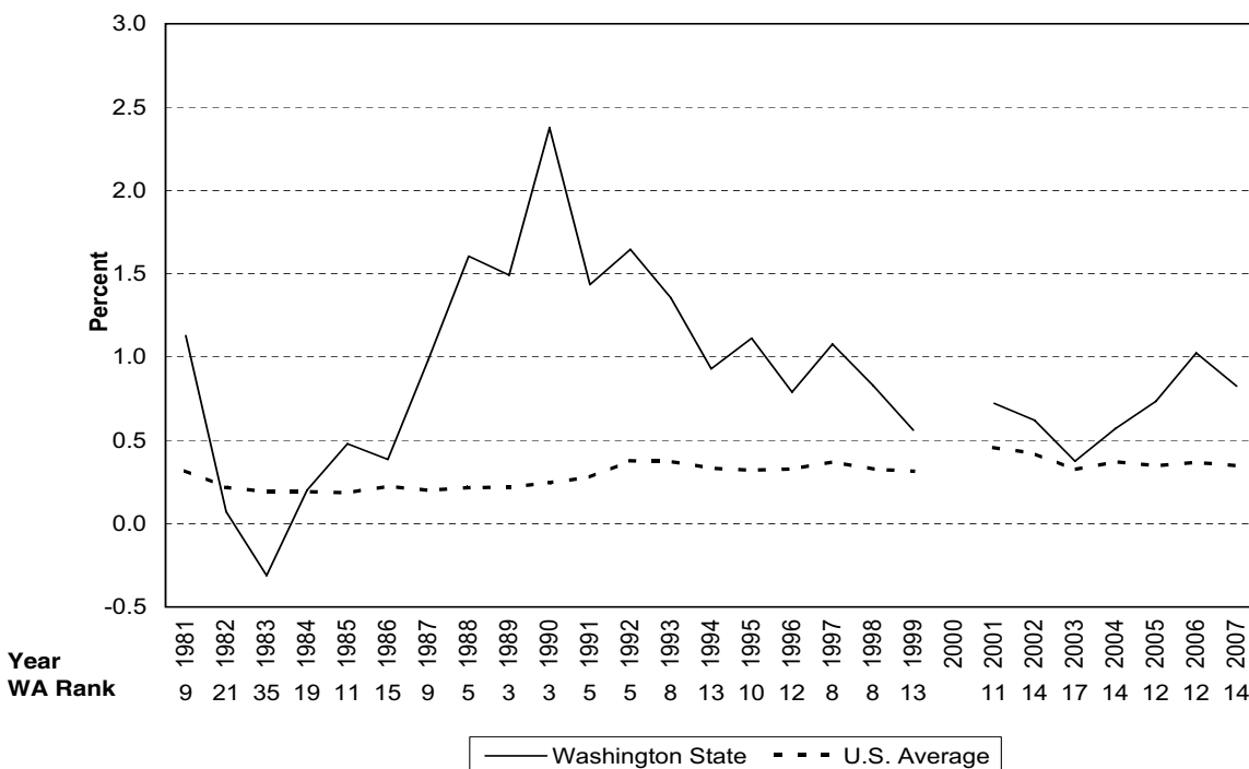
Chart 8 Migration Rate
